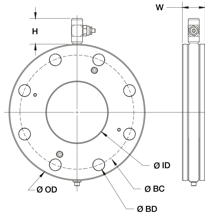
Type 81 Bolt-Thru Isolation Ring
