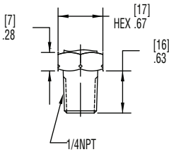
1/4NPT Male Standard
