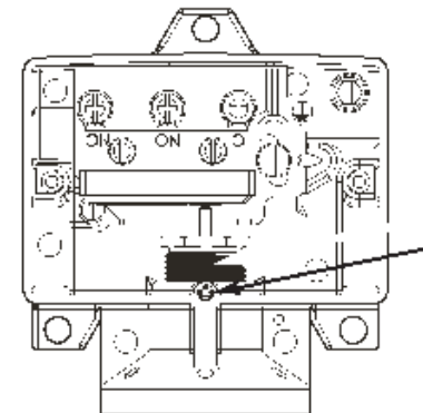
Picture 2 Setpoint locking screw.
