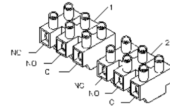
Picture 1 Terminal block. 1 Front switch A 2 Rear switch B
