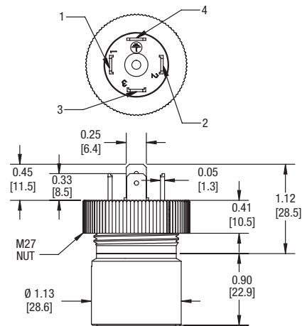
EN 175301-803 Form A CODE: 00DN
