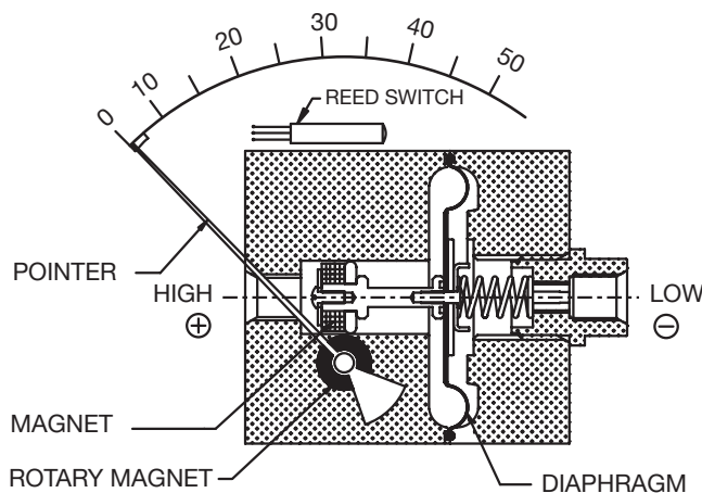
Model 1133/1143 Large Convoluted Diaphragm
