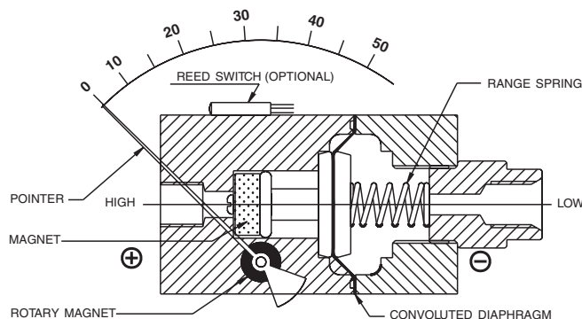
Model 1132 Small Convuluted Diaphragm
