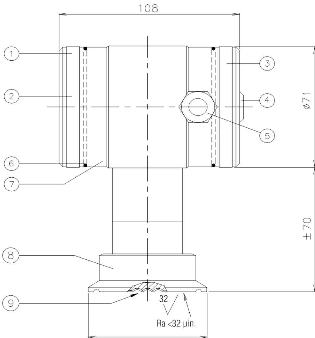
1,5" or 2" TRI CLAMP
