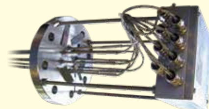
CONVENTIONAL MULTIPOINT THERMOCOUPLE WITHOUT SECURITY CHAMBER
